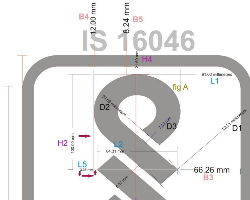
All dimensions in Millimeters
